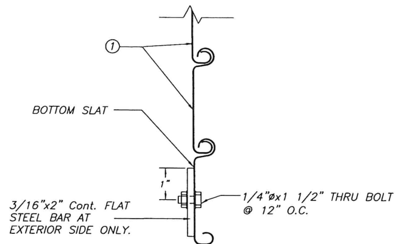
SECTION X1
